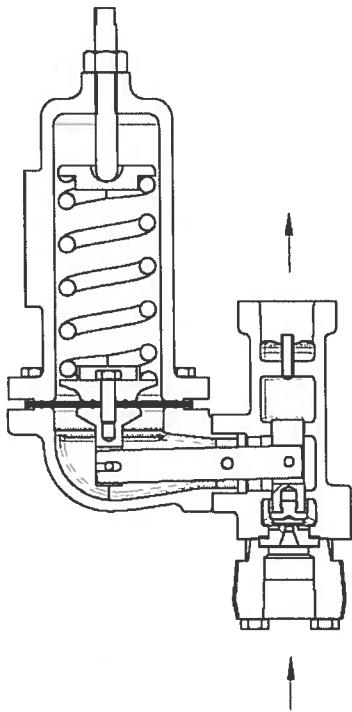
TYPE 630 REGULATOR OPERATIONAL SCHEMATIC
