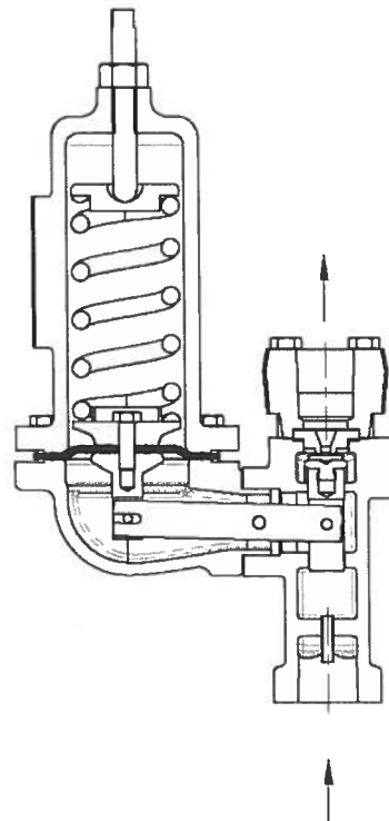
TYPE 630R RELIEF VALVE OPERATIONAL SCHEMATIC
