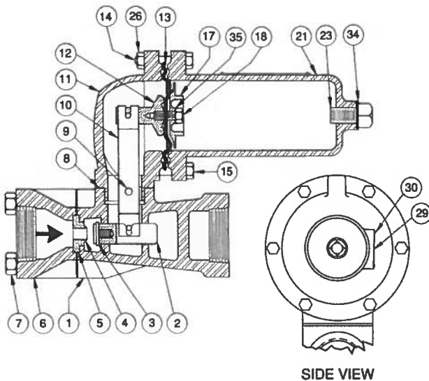
Figure 2: Pressure-Loaded CVS Type 630 Regulator High Pressure Connection
